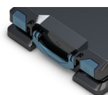
O&O BlueCon
