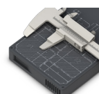
O&O DiskStat
